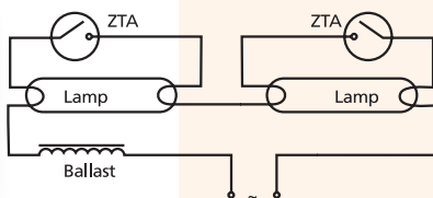
SERIES 220-240 V~
