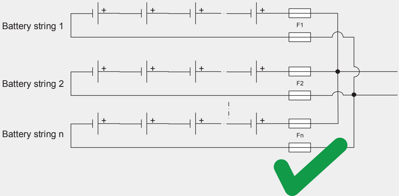
Battery array
